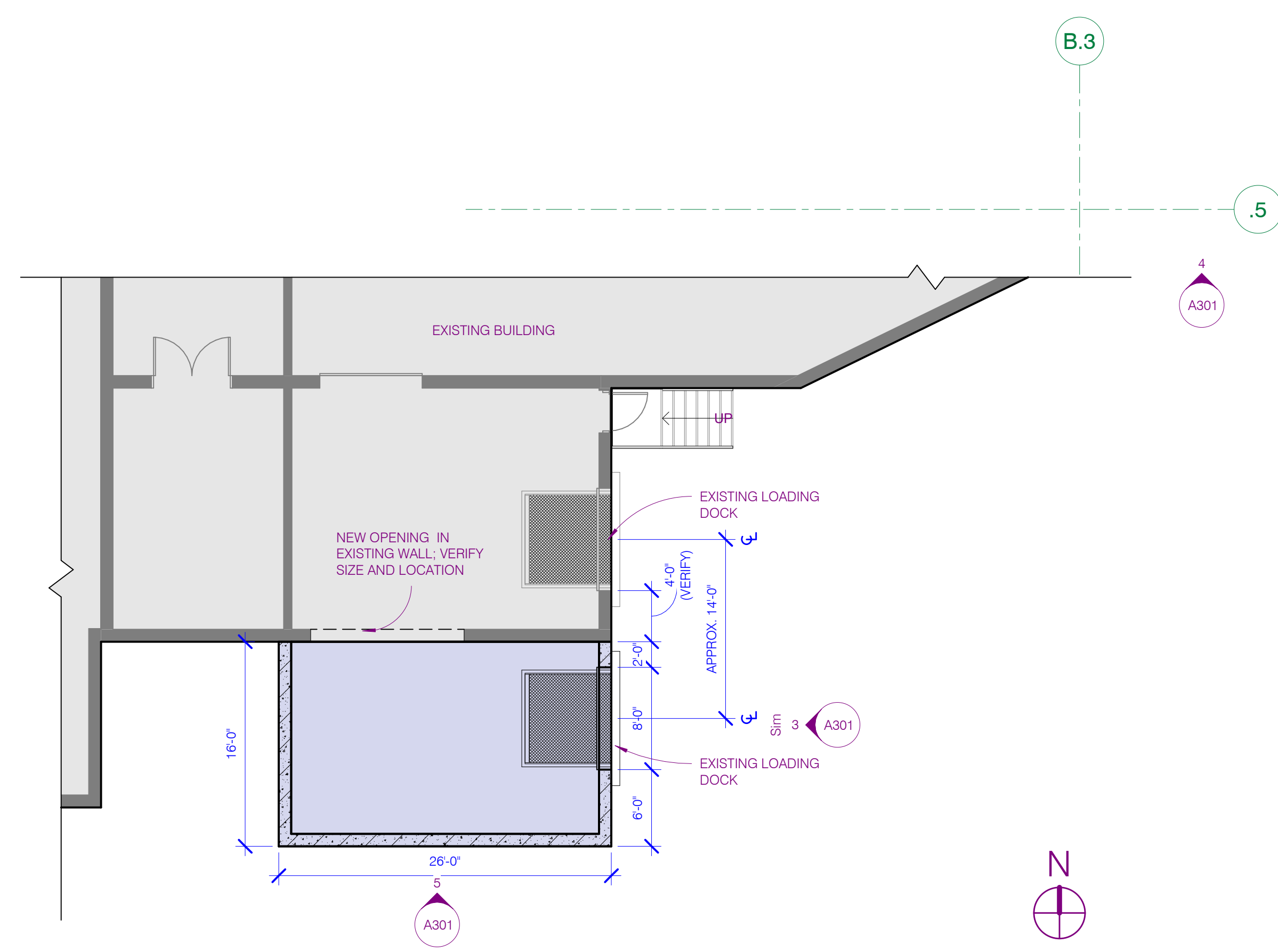
2 LEVEL 2 PLAN - LOADING DOCK A102 1/8" = 1'-0"
