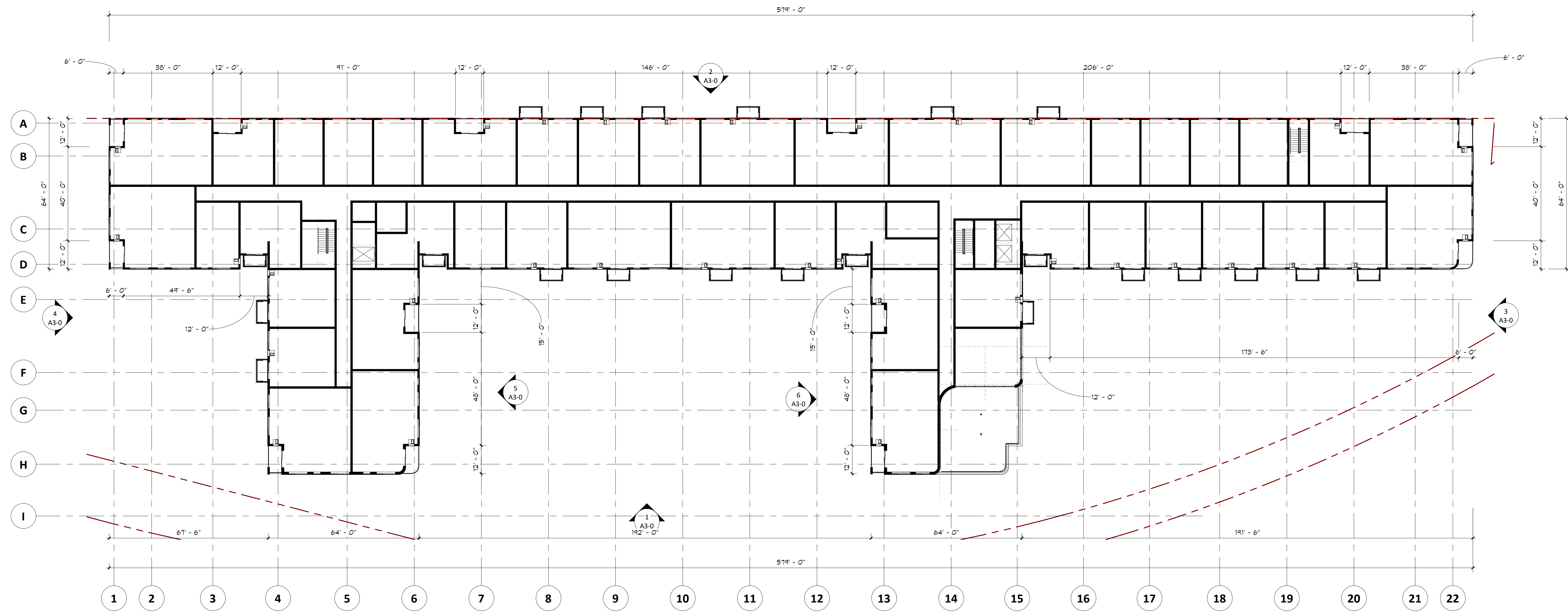
2 LEVEL 6 A1-2 3/64" = 1'-0"
