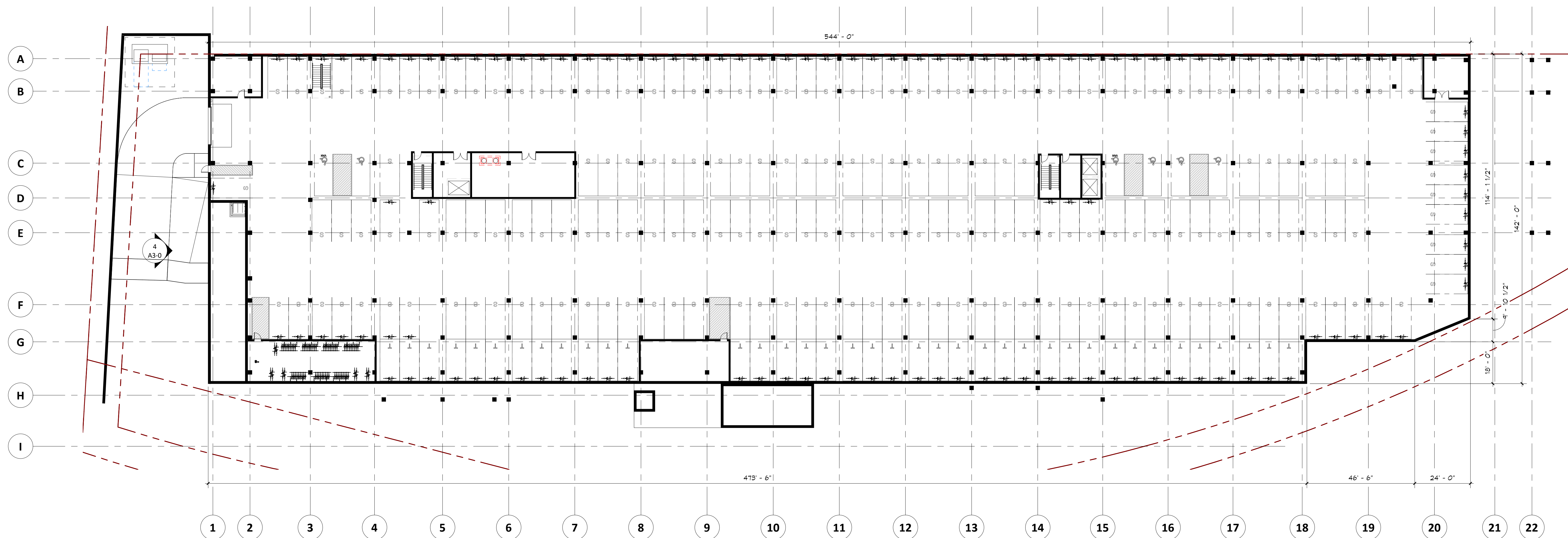
1 LOWER LEVEL A1-0 3/64" = 1'-0"
