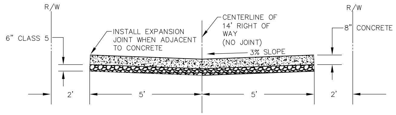
CROSS SECTION OF ALLEY NOT TO SCALE
