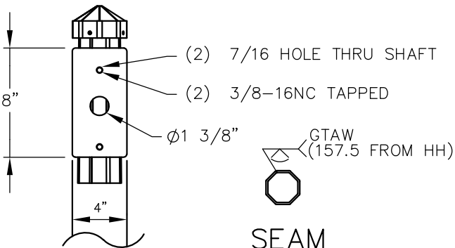
PLATE MTG DETAIL
