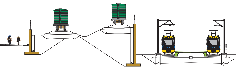
TYPICAL SECTION AT PLATFORM
